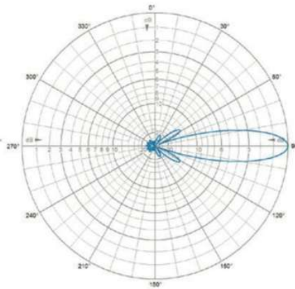
380-470MHz Vertical Pattern
