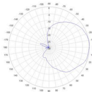
Vertical Beamwidth
